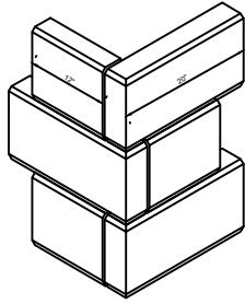
STAGGERED BEVEL (BVS)
